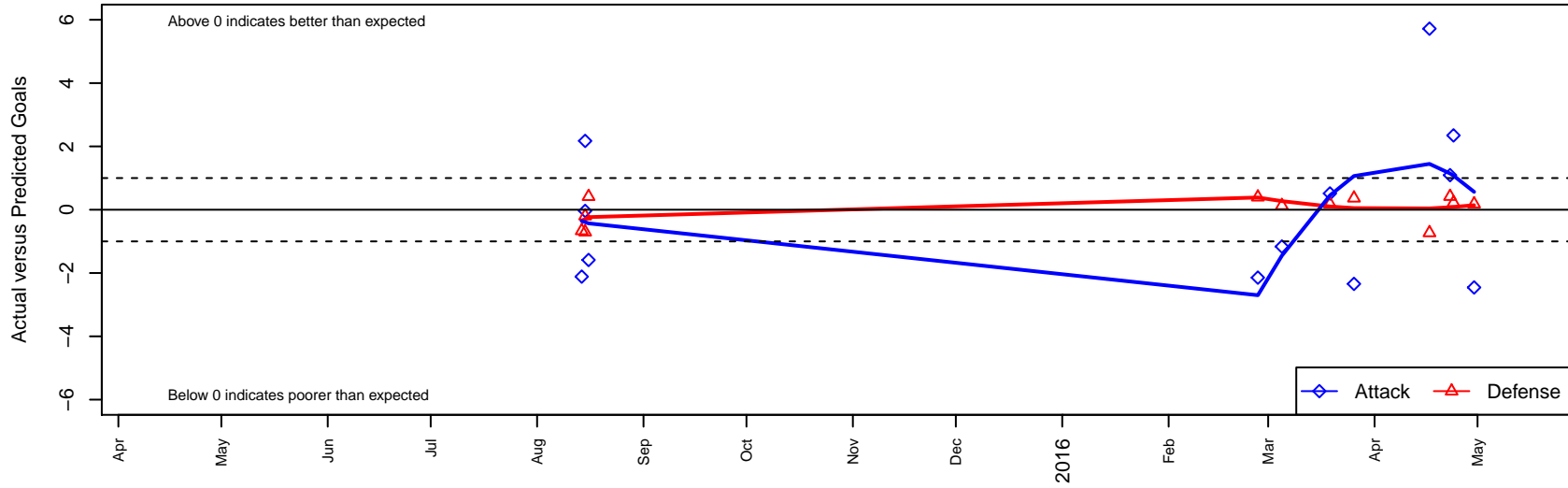
FC Salmon Creek Flower Power G04 Dots are actual minus expected GF (blue circles) and GA (red triangles). Blue line is smoothed change in attack strength. Red is smoothed change in defense strength.
